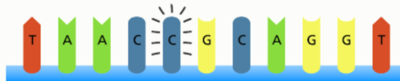
Point mutation
