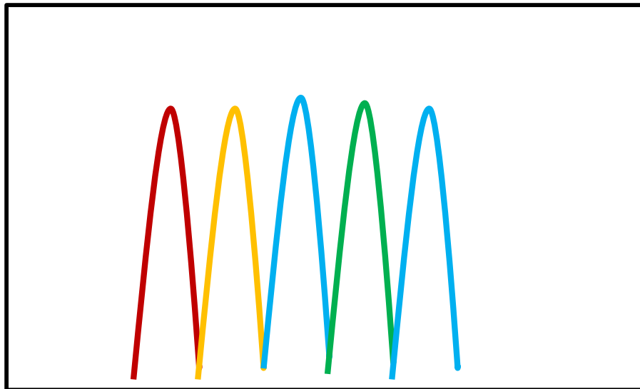
Electropherogram
