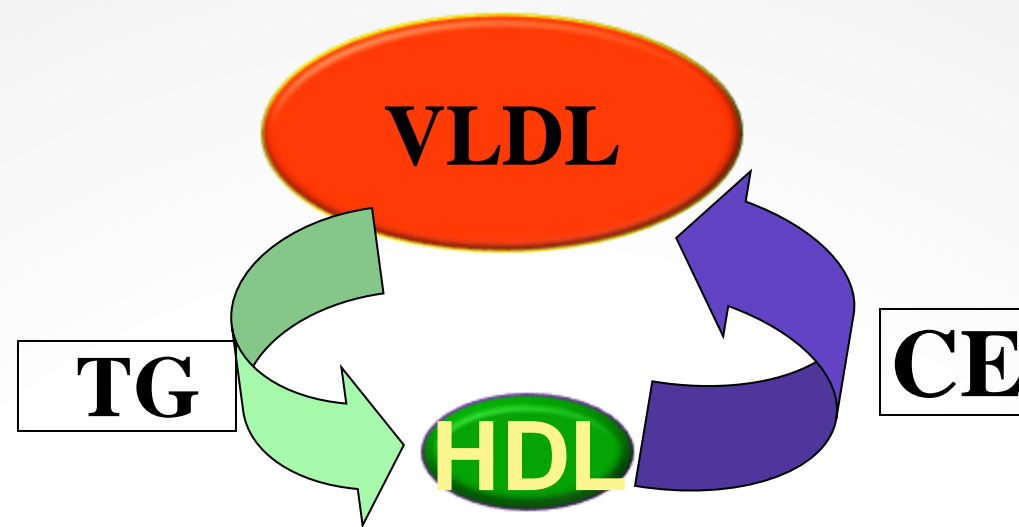
Cholesteryl Ester Transfer Protein (CETP)
