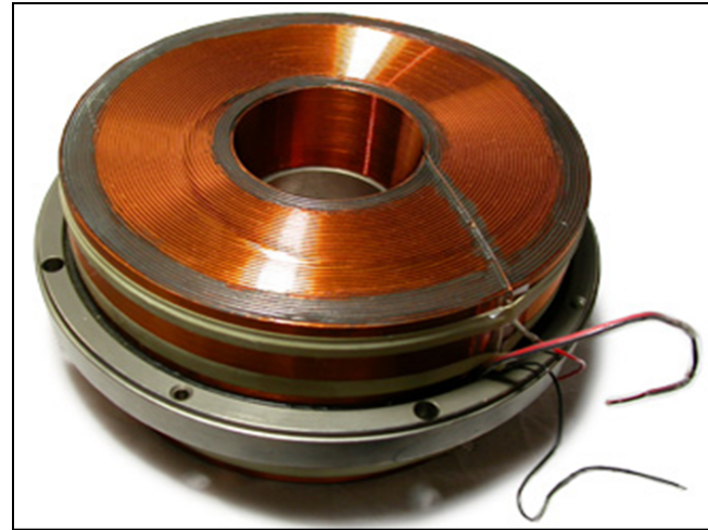
Electromagnetic lens
