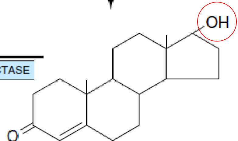
TESTOSTERONE
