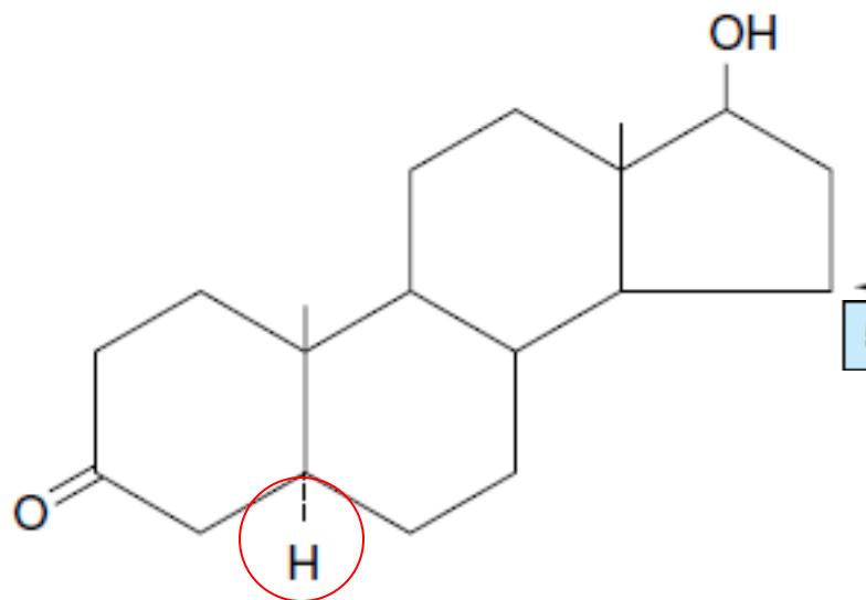
DIHYDROTESTOSTERONE (DHT)
