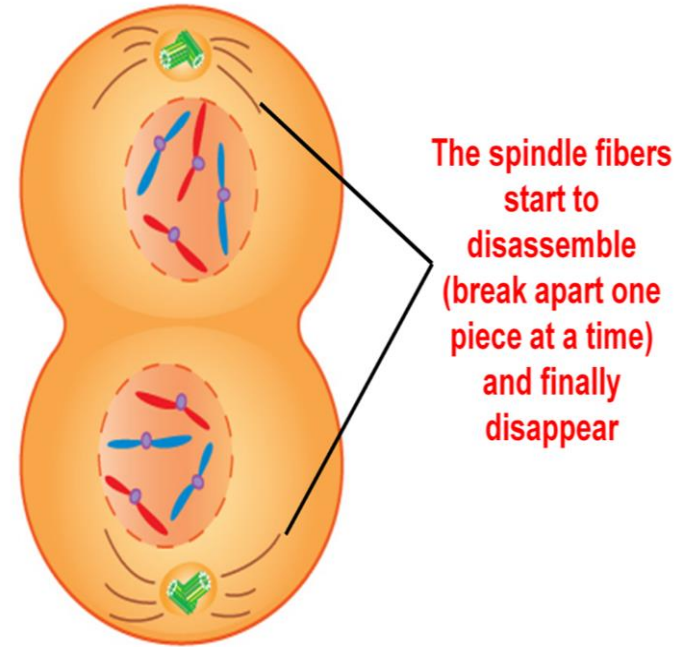
Telophase
