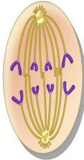
Anaphase
