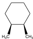
cis-1,2-dimethylcyclohexane
