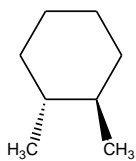
trans-1,2-dimethylcyclohexane
