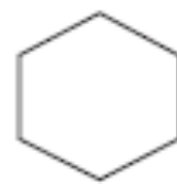
cyclohexane bp 80.7^{\circ}\text{C}
