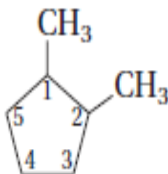
1,2-dimethylcyclopentane (not 1,5-dimethylcyclopentane)
