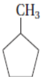
methylcyclopentane (not 1-methylcyclopentane)
