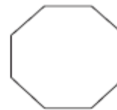
cyclooctane bp 149^{\circ}\text{C}
