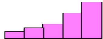
Negatively Skewed
