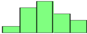
Small Variability
