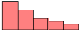
Positively Skewed
