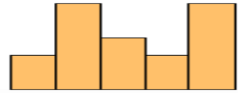
Large Variability
