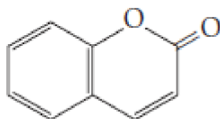
coumarin mp 71°C
