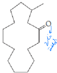
muscone (musk deer) bp 327–330°C
