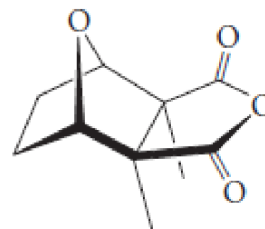
cantharidin mp 218°C
