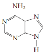
adenine mp 360–365°C (decomposes)
