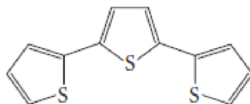
\alpha -terthienyl mp 92–93°C
