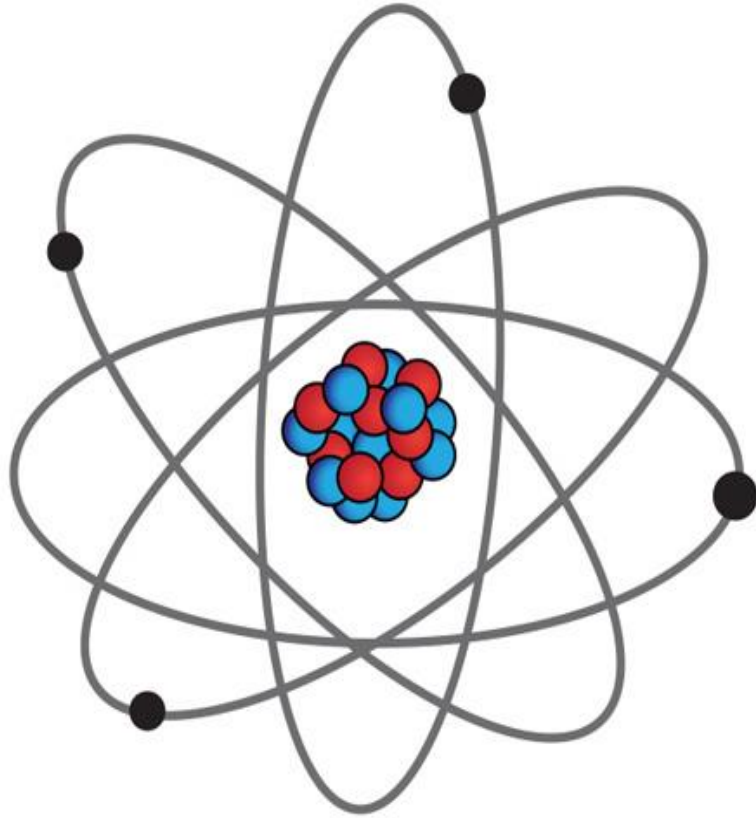
Atom (stable)
