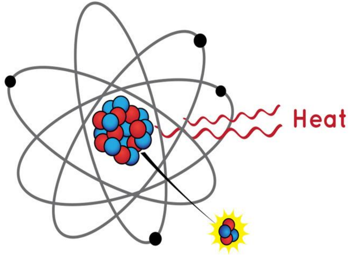
Radioisotope (unstable)
